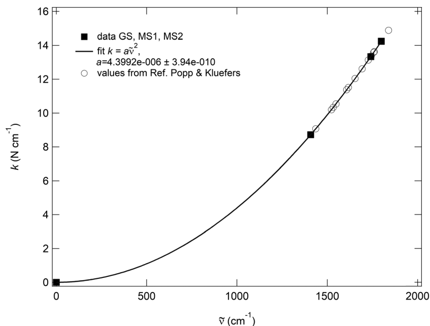
Fig. 7 Quadratic dependence k^{\text{dc}} = a(\tilde{\nu}^{\text{dc}})^2 , ( a = 4\pi^2c^2\mu ) for the NO stretching vibration of GS, MS1, and MS2 in \text{K}_2[\text{RuCl}_5\text{NO}] , resulting from the decoupling into two-atomic harmonic oscillators. For the fit, the point k = \tilde{\nu} = 0 has been added.
