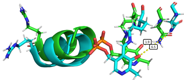
Fig. 6 Overall structural changes following decooordination of Cys52 and rotation of Arg266. The initial structure at 0 ns is shown in green and a snapshot after 1000 ns is shown in blue (species F , chain A ). The bond length d(\text{N}\delta_{\text{Asn149}}-\text{O12}_{\text{PLP}}) is highlighted in the figure, increasing from 1.9 Å (at 0 ns) to 6.5 Å (at 1000 ns). This figure was generated by \alpha -carbon backbone alignment in PyMOL. 86
