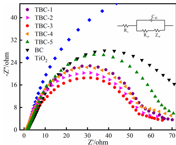
Fig. 7 EIS Nyquist plots of the as-prepared BC, \text{TiO}_2 , and TBC samples in 1 M \text{Na}_2\text{SO}_4 solution and the inset shows the equivalent circuit fitting of EIS data.
