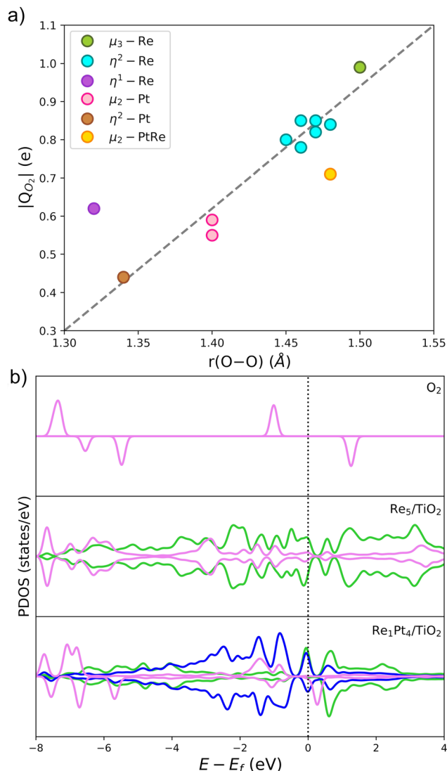
Fig. 6 Electronic properties for \text{O}_2 activation on metal cluster sites. (a) Relationship between \text{O}_2 charge and O–O length for \text{O}_2 adsorption on \text{Re}_n\text{Pt}_m systems. These data correspond to the most stable sites on the gas-phase and supported clusters. (b) The projected density of states (PDOS) of the \text{O}_2 adsorption on \text{Re}_5 and \text{Re}_1\text{Pt}_4 supported clusters. The first panel shows the PDOS of gas-phase \text{O}_2 , and the two panels below are the PDOS for the systems with higher and lower adsorption energy. The 5d states of Re, 5d states of Pt, and 2p states of \text{O}_2 are represented by green, blue, and pink, respectively.
