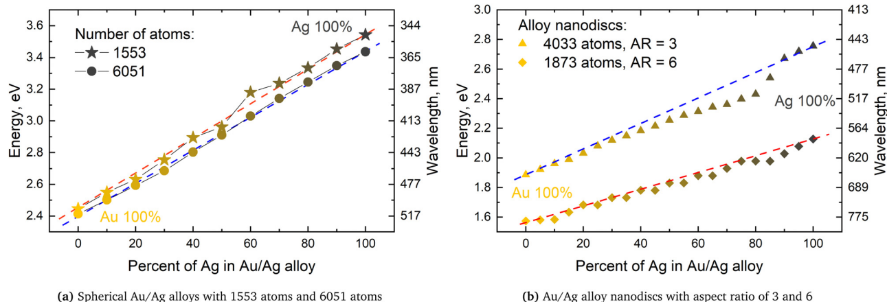
Fig. 12 Position of SPR versus percentage of Ag atoms for Au/Ag alloys of different geometries. Dashed lines indicate Vegard's law. Note that the frequency in wavelength scale is non-linear. From ref. 149.
