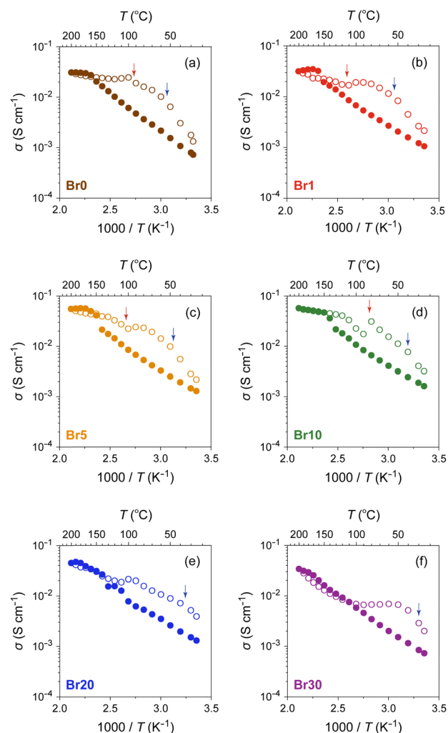
Fig. 6 Temperature dependence of \sigma for \text{AgI-AgBr/MPA} composites with various \text{AgI}:\text{AgBr} molar ratios ((a) Br0 , (b) Br1 , (c) Br5 , (d) Br10 , (e) Br20 , and (f) Br30 ) in heating (closed circles) and cooling (open circles) processes. The red and blue arrows indicate the onset temperatures of the transition on the high- and low-temperature sides, respectively, in the DSC cooling process (Fig. 3).
