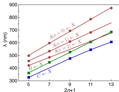
Fig. 3 Wavelengths for the origin transitions of \tilde{\text{A}}^2\Pi_{\text{u/g}} \leftarrow \tilde{\text{X}}^2\Pi_{\text{g/u}} , \tilde{\text{B}}^2\Pi_{\text{u/g}} \leftarrow \tilde{\text{X}}^2\Pi_{\text{g/u}} and \tilde{\text{C}}^2\Pi_{\text{u/g}} \leftarrow \tilde{\text{X}}^2\Pi_{\text{g/u}} band systems for \text{HC}_{2n+1}\text{H}^+ chains plotted against the number of carbon atoms ( 2n+1 ). Wavelengths for the progression members in the acetylenic \text{C}\equiv\text{C} stretch mode are also plotted for the \tilde{\text{A}}^2\Pi_{\text{u/g}} \leftarrow \tilde{\text{X}}^2\Pi_{\text{g/u}} band system. Note that as the chains become longer, overtone vibrational levels (2 quanta of the acetylenic \text{C}\equiv\text{C} stretch mode) associated with the \tilde{\text{A}}^2\Pi_{\text{u/g}} state come into resonance with the vibrationless level of the \tilde{\text{B}}^2\Pi_{\text{u/g}} manifold leading to complications in the spectra. The average energy for transitions in the region of the \tilde{\text{B}}^2\Pi_{\text{u/g}} \leftarrow \tilde{\text{X}}^2\Pi_{\text{g/u}} origin transition are plotted for \text{HC}_9\text{H}^+ , \text{HC}_{11}\text{H}^+ and \text{HC}_{13}\text{H}^+ .
