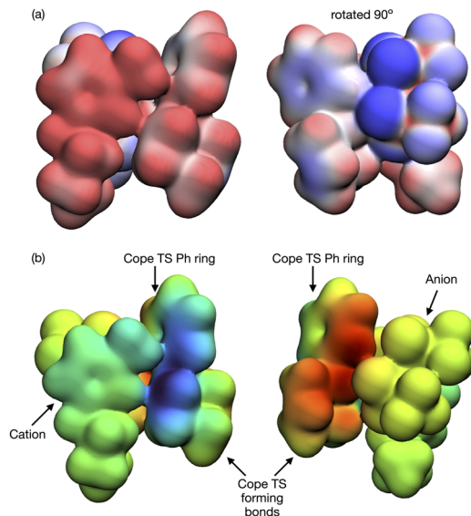
Fig. 13 Reaction B TS-[C 4 C 1 C 1 im][NTf 2 ] (a) electrostatic potential (ESP) mapped onto the 0.007 density iso-surface, red positive, blue negative, maximum \pm 0.05 a.u., (b) \Delta\rho = \text{ESP}_{\text{cluster}} - (\text{ESP}_{\text{TS}} + \text{ESP}_{\text{solvent}}) mapped onto the 0.007 a.u. (e/a_0^3) density iso-surface. "Rainbow" colour scheme, blue = negative, green = neutral, red = positive, maximum \pm 0.02 a.u.
