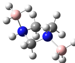
Fig. 2 The optimized structure of IMBB at M06-2X/cc-pVQZ level.
