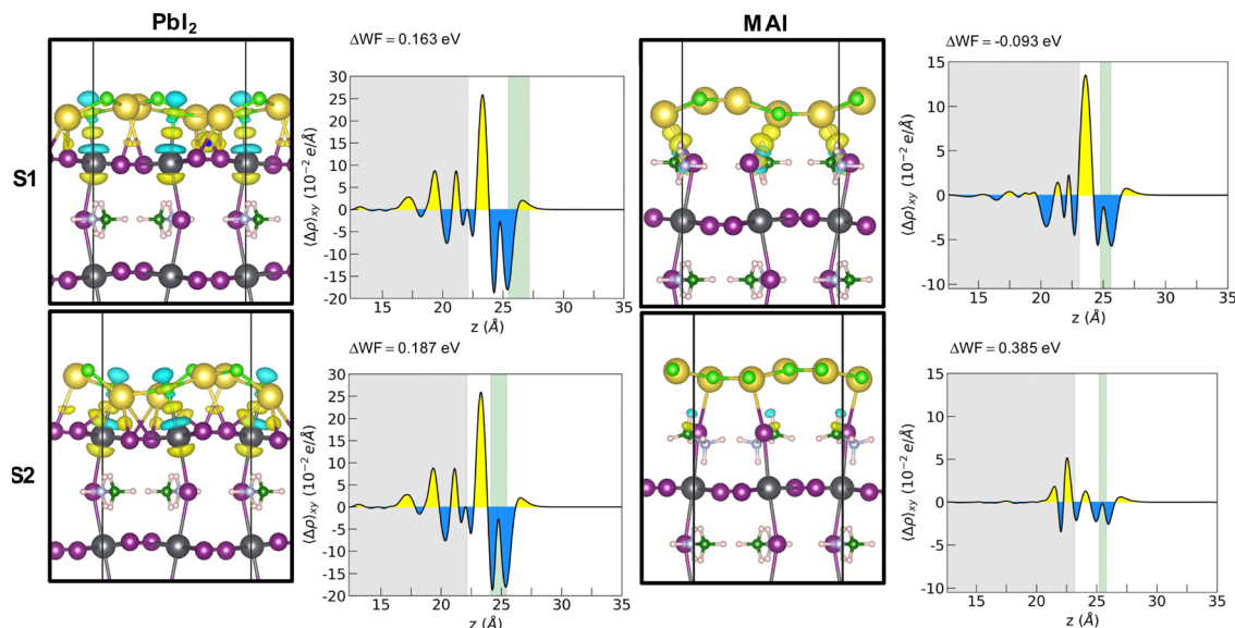
Fig. 3 Electron density differences for the interaction between the \text{PbI}_2 - and the MAI-terminated MAPI film and the NaCl layer (left). Yellow denotes increased electronic density and light blue indicates decreased electronic density. Isosurface value: 0.0025. Planar average charge density difference for each system (right). Color code: Pb – dark gray; I – violet; C – green; N – light blue; H – light pink; Na – yellow; Cl – light green.
