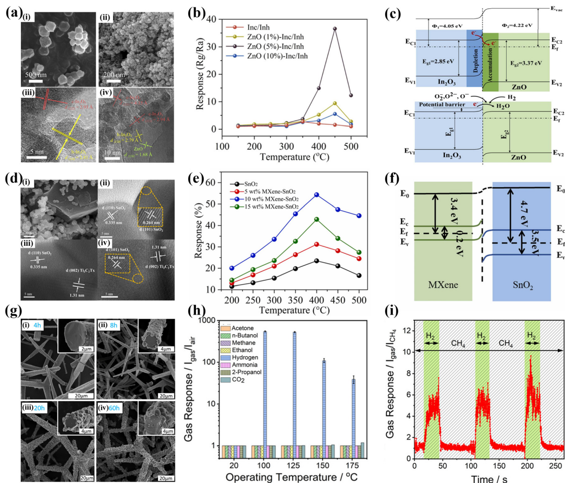
Fig. 9 (a) SEM images of (i) ZnO and (ii) Inc/Inh; HRTEM images of (iii) Inc/Inh and (iv) ZnO-Inc/Inh. (b) Response of Inc/Inh-based sensors to 2000 ppm \text{H}_2 at different operating temperatures ranging from 100 to 500 °C. (c) Sensing mechanism of the heterojunction between \text{In}_2\text{O}_3 and ZnO. Reproduced with permission from ref. 117. Copyright 2024 Elsevier. (d) (i) SEM image of 10 wt% MXene-SnO 2 , (ii) HRTEM image of SnO 2 , and (iii) and (iv) HRTEM image of 10 wt% MXene-SnO 2 . (e) Response of SnO 2 -based sensors to 600 ppm \text{H}_2 at different operating temperatures ranging from 200 to 500 °C. (f) Schematic diagram of the heterojunction between MXene and SnO 2 . Reproduced with permission from ref. 119. Copyright 2024 Elsevier. (g) SEM images of t-ZnO@ZIF-8 at different reaction times of 4, 8, 20, and 60 h. (h) Selectivity of the t-ZnO@ZIF-8 (4 h)-based sensor to 100 ppm of different gases at different operating temperatures on log 10 scales. (i) Response-recovery curve of t-ZnO@ZIF-8 (4 h) to 100 ppm \text{H}_2 in \text{CH}_4 at 100 °C. Reproduced with permission from ref. 120. Copyright 2023 American Chemical Society.
