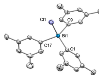
Fig. 3 Solid state structure of 10. Ellipsoids are drawn at the 50% probability level. H atoms and \text{BAR}^{\text{F}} are omitted for clarity. Selected bond lengths (Å) and angles ( ^\circ ): Bi1–Cl1: 2.4028(8), Bi1–C1: 2.185(3), Bi1–C9: 2.180(3), Bi1–C17: 2.189(3), C1–Bi1–C9: 121.63(11) , C1–Bi1–C17: 111.32(10) , C9–Bi1–C17: 112.55(11) .
