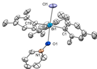
Fig. 5 Solid state structure of 13 . Ellipsoids are drawn at the 50% probability level. H atoms and BARF are omitted for clarity. Selected bond lengths (Å) and angles (°): Bi1–Cl1: 2.507(7), Bi1–O1: 2.404(6), Bi1–C1: 2.229(6), Bi1–C10: 2.226(5), Bi1–C19: 2.236(6), N1–O1: 1.334(8), C1–Bi1–C10: 117.9(2), C1–Bi1–C19: 121.7(2), C10–Bi1–C19: 119.3(2), Cl1–Bi1–O1: 173.5(2), N1–O1–Bi: 136.7(4).
