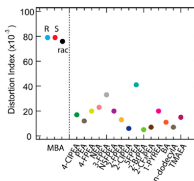
Fig. 23 D values of (R/S\text{-}Rac\text{-MBA})_2\text{SnI}_4 and of other Sn-I layered HOIPs reported in the literature. Reprinted with permission from ref. 42 Copyright©2020 American Chemical Society.
