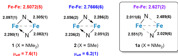
Fig. 2 Summary of distances (Å) in the Fe_2N_2 core in 1 , 2 , and 1a and comparison to the RT \mu_{eff} values in \mu_B (susceptibility balance). Distances for 1a are shown for one of two crystallographically unique complexes in the asymmetric unit cell, but they are representative of both complexes.
