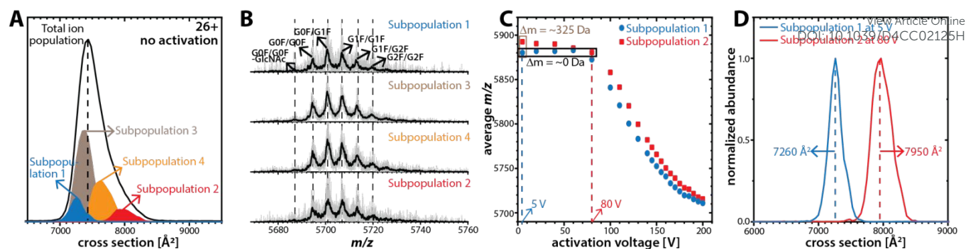
Figure 2. Structural heterogeneity of NISTmAb probed by non-ensemble Tandem-TIMS measurements. (A) The ion mobility peak of charge state 26+ (black trace) is superimposed with four subpopulations (blue, red, orange, and light brown traces). The subpopulations correspond to distinct collision cross-sections and do not interconvert for at least \sim 100 ms, which indicates that these are kinetically stable species. (B) The mass spectrum of each subpopulation shows six dominant glycoforms with the same m/z and similar relative abundance, indicating that the subpopulations comprise the same glycoforms. (C) The initial average mass difference between subpopulations 1 and 2 is \sim 325 Da. The average m/z of subpopulation 1 at an activation voltage of 5 V is identical to that obtained at 80 V for subpopulation 2 ( m/z \sim 5880 ). (D) Despite having the same mass and, thus, the same number of attached solvent adducts, the subpopulations maintain the differences in their collision cross-sections of \sim 10\% .
