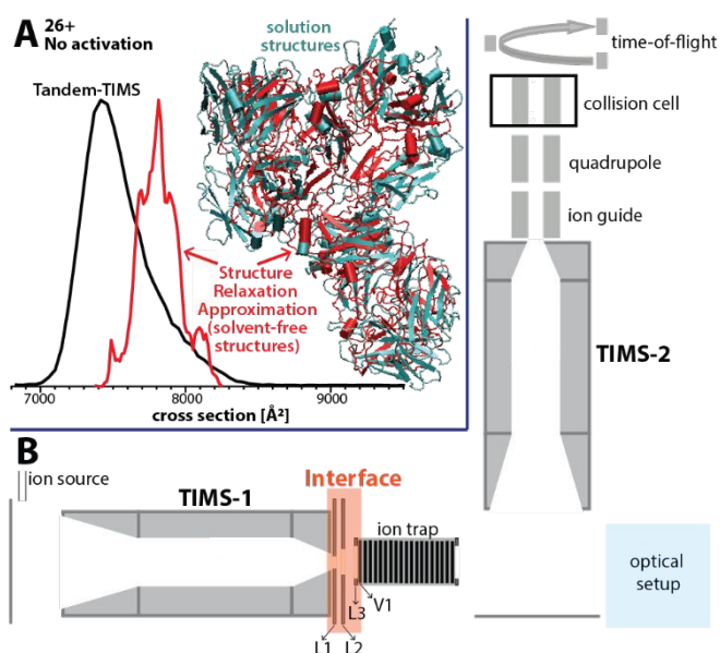
Figure 1. (A) The ion mobility spectrum computed by our computational Structure Relaxation Approximation for NISTmAb (red traces) agrees well with the experimental spectrum (black trace). The representative solvent-free NISTmAb structure computed by the SRA for charge state 26+ (red, cartoon) indicates strong retention of native contacts with respect to the representative structure obtained from explicit solvent molecular dynamics simulations (cyan, cartoon). (B) Schematics of the Tandem-TIMS instrument coupled to a QqTOF mass spectrometer. Tandem-TIMS comprises of two TIMS devices, an interface region with electrodes (L1, L2, L3, V1) capable of applying high electric fields to select and activate analyte ions. (See refs. 14 – 19 for details).
