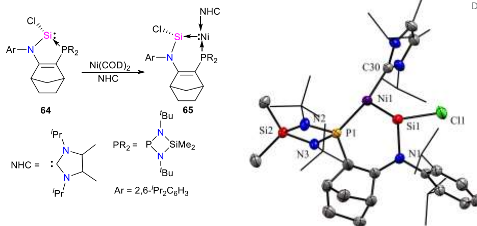
Scheme 23 Synthesis of Ni-stabilized silylene 65 and its molecular structure. Reproduced from Ref [70] Copyright © 2022 Wiley-VCH GmbH
