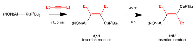
Scheme 8 Experimental insertion of internal 3-hexyne in the Cu–Al bond of the [Bu_3PCuAl(NON)] complex. 68
