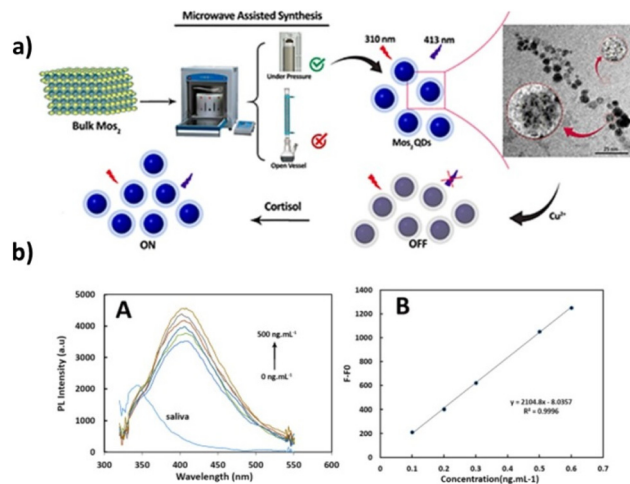
Fig. 5 (a) Schematic representation of the production of highly luminescent \text{MoS}_2 quantum dots (QDs) by microwave exfoliation of the \text{MoS}_2 powder. (b) Fluorescence spectra of the \text{MoS}_2 QDs- \text{Cu}^{2+} on cortisol addition in the range of 0\text{--}500 \text{ ng mL}^{-1} (left), and calibration curve for cortisol ( \lambda_{\text{ex}} = 310 nm and \lambda_{\text{em}} = 413 nm) (right). Adapted from ref. 72 with permission from Elsevier, copyright 2022.
