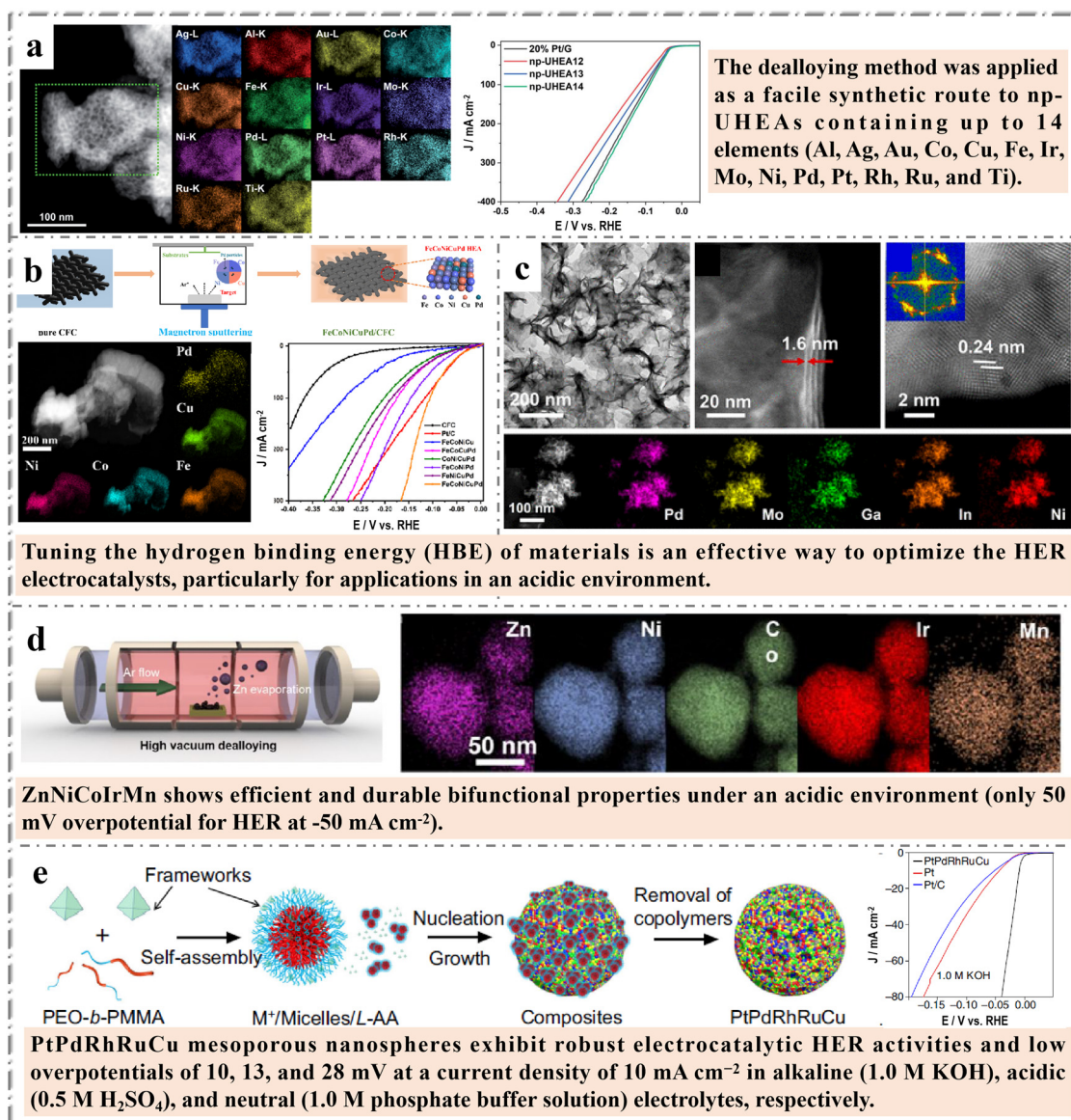
Fig. 5 Examples of HEMs in HER: (a) TEM image, EDX mappings and electrocatalytic performance of np-UHEAs (Al 8 Ag 1 Au 1 Co 1 Fe 1 Ir 1 Mo 1 Ni 1 Pd 1 Pt 1 Rh 1 Ru 1 Ti 1 ). Reprinted with permission. 95 Copyright 2021, The Royal Society of Chemistry. (b) Fabrication schematic illustration, TEM image and corresponding EDX mappings and electrocatalytic performance of the FeCoNiCuPd film. Reprinted with permission. 96 Copyright 2022, Elsevier Ltd. (c) Electron microscopic characterization of high-entropy alloy PdMoGaInNi nanosheets. Reprinted with permission. 97 Copyright 2022, American Chemical Society. (d) Schematic illustration of selective Zn dealloying through vapor dealloying process and EDX mappings of ZnNiCoIrMn). Reprinted with permission. 98 Copyright 2023, Wiley-VCH; (e) Schematic illustration of PtPdRhRuCu mesoporous nanospheres and electrocatalytic performance of samples (polarization curves). Reprinted with permission. 99 Copyright 2023, Springer Nature.
