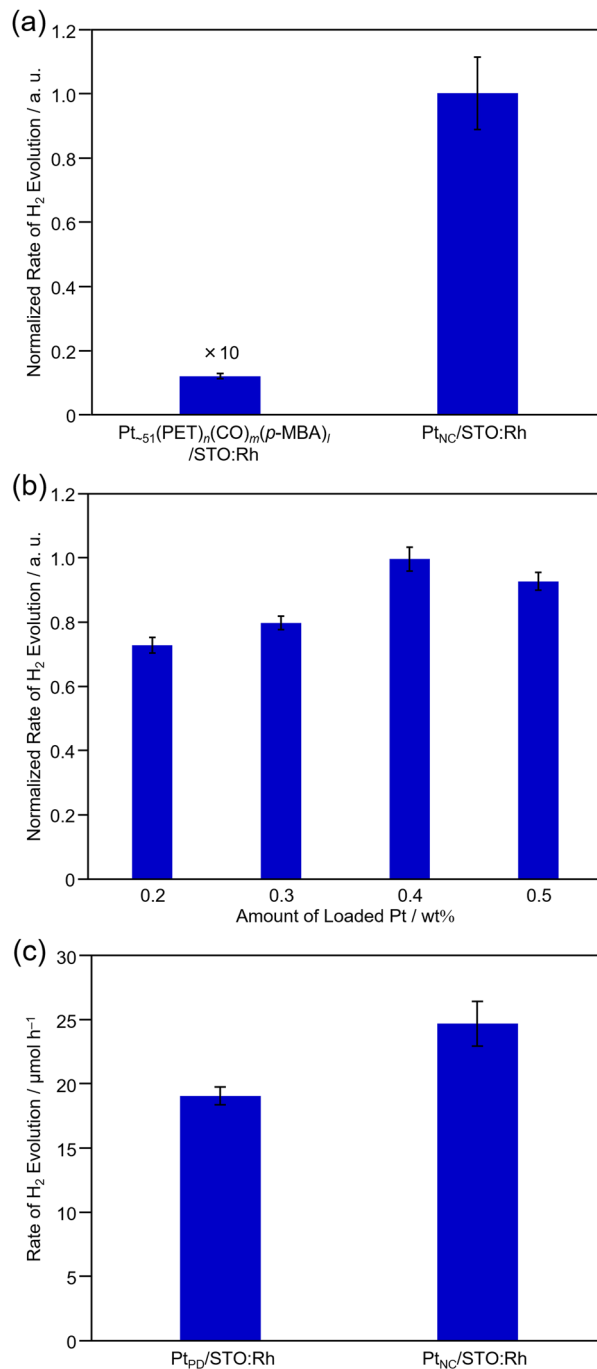
Fig. 5 H 2 -evolution activity of Pt cocatalyst-loaded STO:Rh photocatalysts. (a) Before ( \text{Pt}_{51}(\text{PET})_n(\text{CO})_m(\text{p-MBA})_l/\text{STO:Rh} ) and after ( \text{Pt}_{\text{NC}}/\text{STO:Rh} ) calcination of Pt NC-loaded STO:Rh and (b) dependence of loading weight of the Pt cocatalyst for \text{Pt}_{\text{NC}}/\text{STO:Rh} . (c) Comparison of H 2 -evolution activity between \text{Pt}_{\text{NC}}/\text{STO:Rh} and \text{Pt}_{\text{PD}}/\text{STO:Rh} . In (a) and (c), the loading weight of Pt on them was 0.4 wt%. In order to eliminate the effect of the difference in the activity of each photocatalyst, STO:Rh synthesized in the same batch was used in each experiment (a)–(c).
