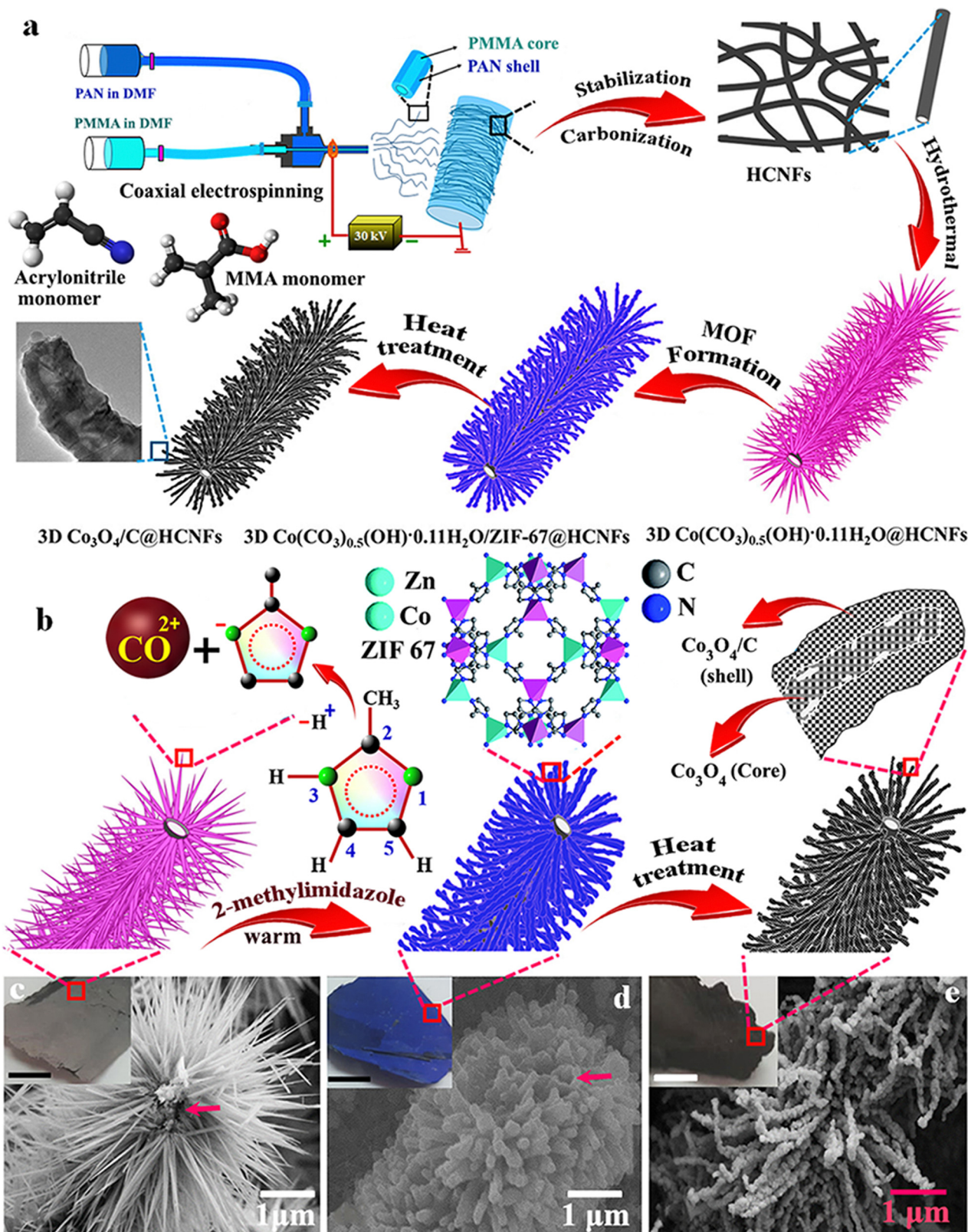
Fig. 14 (a and b) Schematic and mechanism of the fabrication of 3D \text{Co}_3\text{O}_4/\text{C} @HCNF nanocomposites. FE-SEM image of (c) \text{Co}(\text{CO}_3)_{0.5}\text{OH} \cdot 0.11\text{H}_2\text{O} @HCNFs, (d) \text{Co}(\text{CO}_3)_{0.5}\text{OH} \cdot 0.11\text{H}_2\text{O} /ZIF-67@HCNFs and (e) \text{Co}_3\text{O}_4/\text{C} @HCNFs. Reproduced from ref. 121 with permission from American Chemical Society, copyright 2020.
