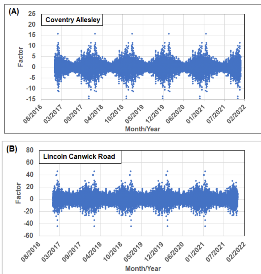
Fig. 4 Seasonal derivative ( t - 12 to t - 1 ) ( SD ) calculated from hourly NOx air quality datasets from 2017 to 2021 for two example recording stations in Central England Cities: (A) Coventry Allesley (urban background site); and, (B) Lincoln Canwick Road (urban roadside site). This trend-attribute variable captures a dimension of seasonality that can be used effectively by the NOx prediction models.
