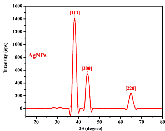
Fig. 3 The XRD pattern of the AgNPs.
