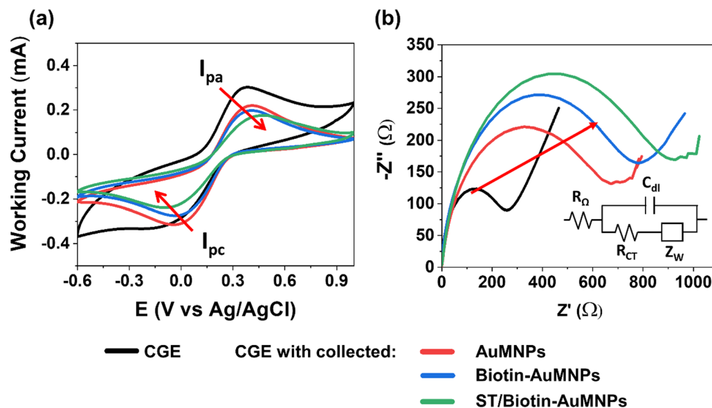
Fig. 2 (a) Cyclic voltammetry and (b) Nyquist plots for bare CGE, CGE with collected AuMNP, CGE with collected biotin-AuMNP and CGE with collected ST/biotin-AuMNP ( [\text{ST}] = 10^{-10} M). All the electrochemical measurements were carried out in a three-electrode configuration using a 0.1 M KCl aqueous solution containing 10 mM [\text{Fe}(\text{CN})_6]^{3-/4-} as redox probe.
