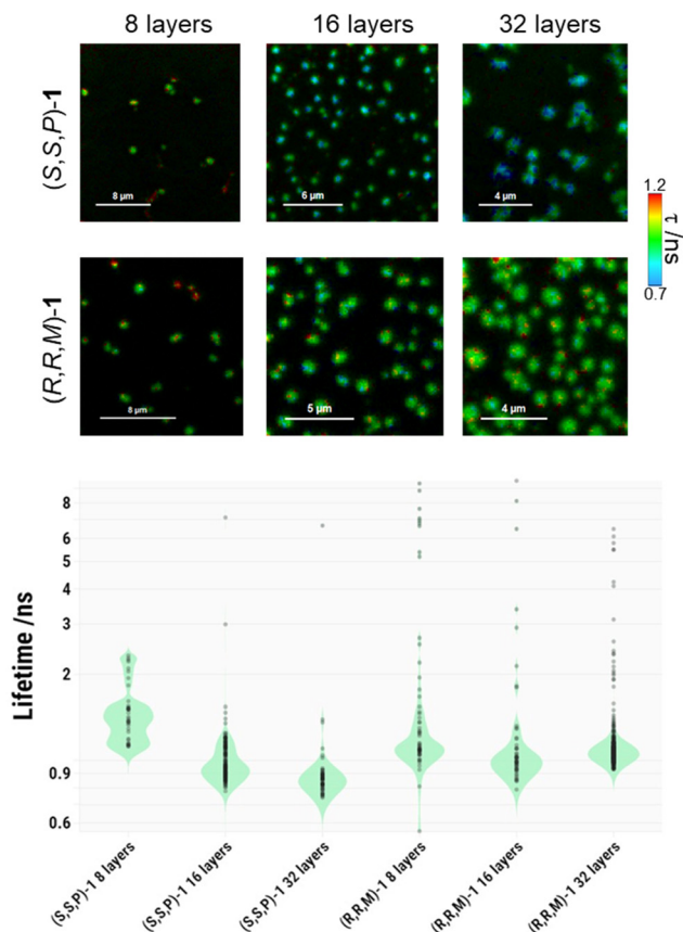
Fig. 5 Representative FLIM images of compounds (S,S,P)-1 and (R,R,M)-1 transferred onto glass slides after subsequent deposition of 8, 16, or 32 layers; and the corresponding violin plot of the particle-wise analysis from, at least, 3 different images in each case.
