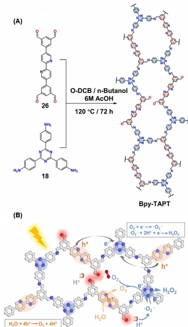
Fig. 15 (A) Sub-stoichiometric synthesis of the COF Bpy-TAPT from the monomers 26 and 18, showing the presence of unreacted aldehyde sites. (B) Photocatalytic generation of \text{H}_2\text{O}_2 from water using Bpy-TAPT and its postulated mechanism. Reproduced from ref. 133 with permission from Elsevier, copyright 2023.
