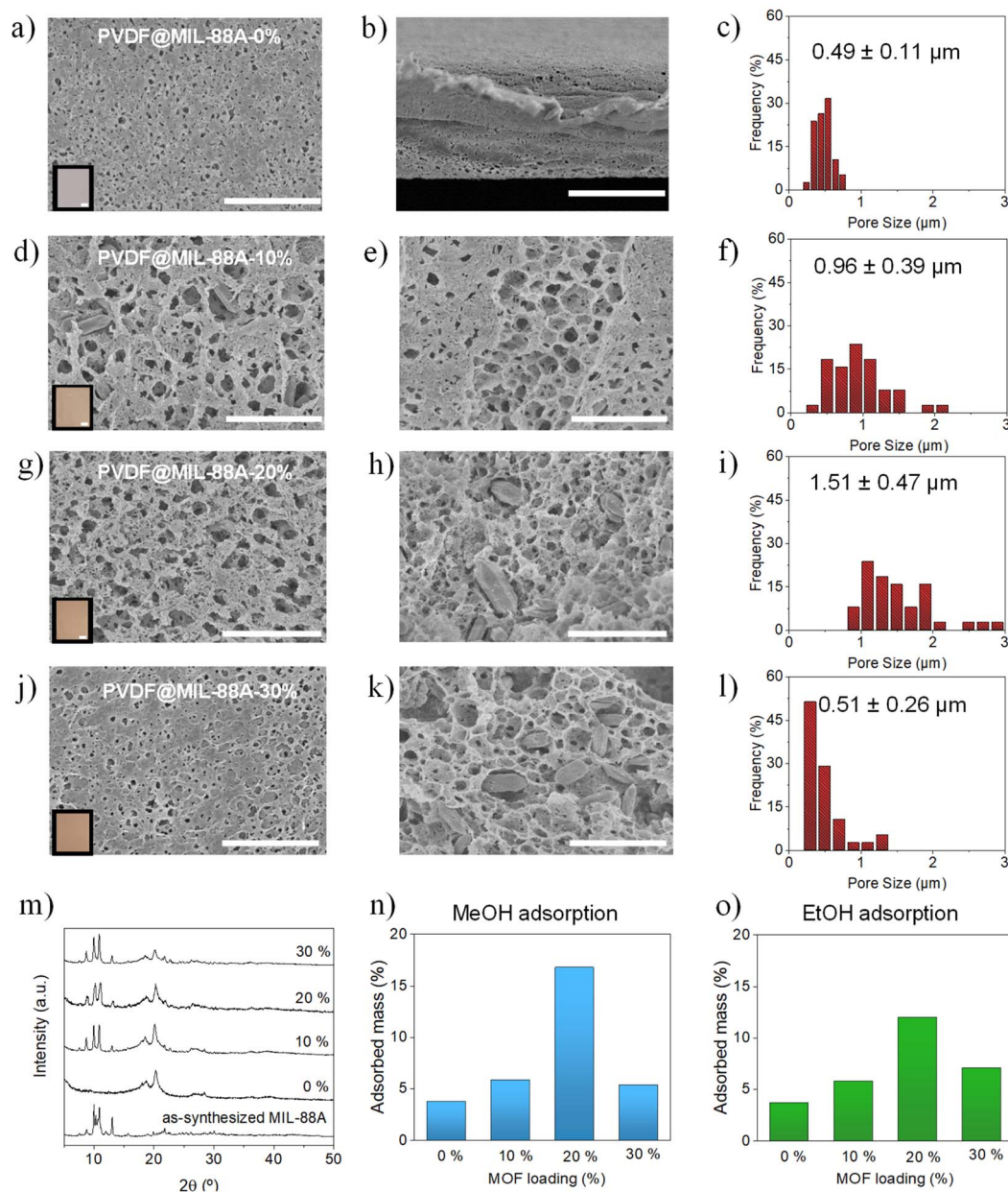
Fig. 8 SEM images (scale bar: 10 \mu\text{m} ) for pore size and morphology characterization of PVDF@MIL-88A membranes and captured images (inset figure, scale bar: 1 cm) with different MOF loadings: (a, d, g, j) surface, (b, e, h, k) cross section and (c, f, i, l) pore-size distribution and average pore size of 0, 10, 20 and 30 wt% MOF-loaded membranes, respectively. (m) PXRD of MIL-88A(Fe) and prepared membranes. Adsorption of alcohols from water in PVDF@MIL-88A(Fe) membranes: (n) methanol and (o) ethanol.
