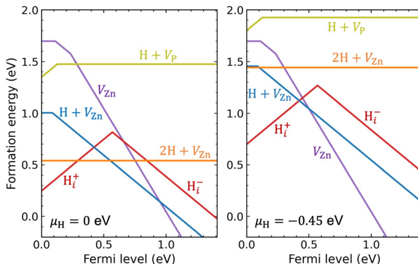
Fig. 4 Formation energies as a function of Fermi level for hydrogen interstitial ( H_i ) and hydrogen-vacancy complexes, including the H + V_{\text{P}} , 2H + V_{\text{Zn}} , and H + V_{\text{Zn}} , in \text{Zn}_3\text{P}_2 , under Zn-poor/P-rich condition and at two different chemical potentials of H ( \mu_{\text{H}} ): the H-rich limit \mu_{\text{H}} = 0 eV (left panel) and a lower \mu_{\text{H}} at -0.45 eV (right panel). For comparison the formation energy of V_{\text{Zn}} is also depicted.
