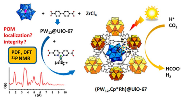
Scheme 8 Scheme for photocatalytic reduction of \text{CO}_2 to produce formate catalyzed by (\text{PW}_{12}\text{Cp}^*\text{Rh})\text{@UiO-67} . Reprinted from ref. 89 with permission from American Chemical Society (Copyright 2020).
