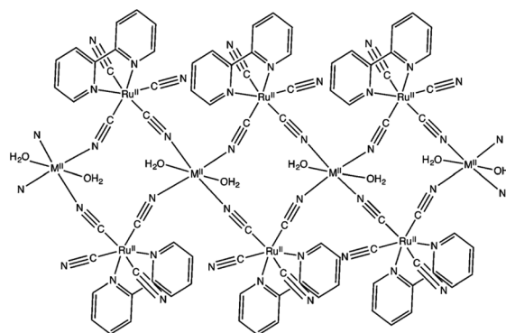
Fig. 1 Schematic structure of M(II)[(bpy)Ru(II)(CN) 4 ] n . Reprinted from ref. 71 with permission from the Royal Society of Chemistry (Copyright 2017).
