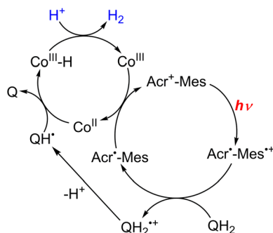
Scheme 20 Proposed mechanism of photocatalytic evolution of H_2 from X-QH 2 with Acr^+-Mes and Co^{III}(dmgH)_2ClPy . Reprinted from ref. 164 with permission from American Chemical Society (Copyright 2020).
