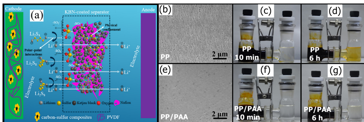
Fig. 3 (a) Schematic of the mechanism of physical confinement of the PS in the porous structure of the KB and polar–polar interaction with \text{SO}_3^- , with Nafion filler 143 (Reproduced with permission from ref. 143. Copyright 2020, Elsevier). SEM of (b) PP and (e) PP/PAA. Digital photograph of a polysulfide diffusion test with a PP separator after (c) 10 min and (d) 6 h and PP/PAA after (f) 10 min and (g) 6 h (h) 166 (Reproduced with permission from ref. 166. Copyright 2018, Elsevier).
