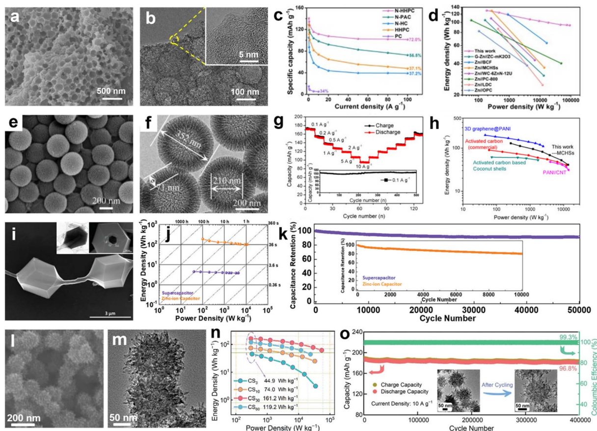
Fig. 9 (a) SEM image and (b) TEM image of the honeycomb-like carbon matrix. (c) Rate performance and (d) Ragone plots of the assembled Zn-ion hybrid capacitors. Reproduced with permission. 164 Copyright 2022, Elsevier. (e) SEM image and (f) TEM image of mesoporous hollow carbon spheres and their (g) rate performance and (h) Ragone plot for Zn-ion capacitors. Reproduced with permission. 165 Copyright 2020, Elsevier. (i) SEM image, (j) Ragone plots, and (k) cycling performance of a necklace-like tubular 3D carbon framework cathode. Reproduced with permission. 168 Copyright 2020, Wiley-VCH. (l) SEM image and (m) TEM image of carbon superstructures and corresponding (n) Ragone plots and (o) cyclability. Reproduced with permission. 114 Copyright 2022, Wiley-VCH.
