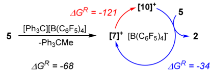
Scheme 3 Catalytic cycle for the transformation of germa-adamantane 5 into its isomer 2 initiated by trityl tetrakis-pentafluorophenylborate. Free reaction enthalpies \Delta G^{\text{R}} are given in italics (calculated at M06-2X/6-311+G(d,p)).
