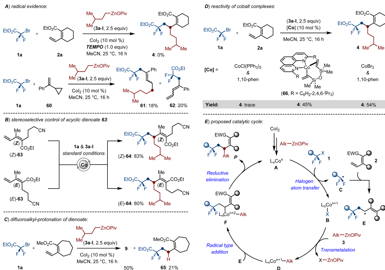
Scheme 6 Mechanistic studies.
