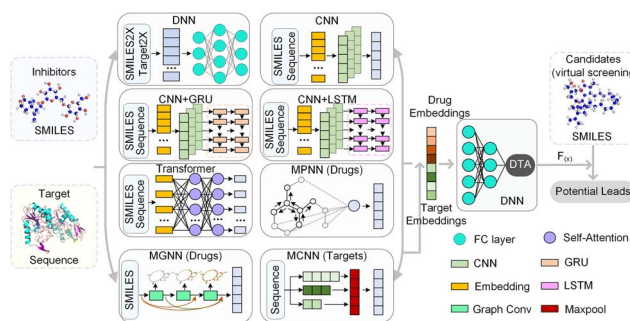
Fig. 6 The framework of the HNN-based EL model for DTA prediction. SMILES2X and Target2X represent 4 different descriptors of drugs and targets respectively. The HNN-based EL model integrates multiple basic models to effectively extract embedding features of drugs and targets and predict their DTA. The trained HNN is used to further screen and identify drug candidates for potential leads to activate or inhibit targets.
