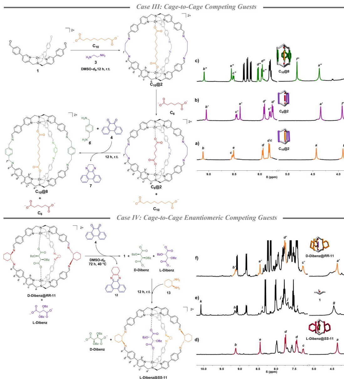
Fig. 2 Case III: partial ^1\text{H} -NMR ( \text{DMSO-}d_6 , 500 MHz) of (a) \text{C}_{10}\text{@}2 , (b) \text{C}_6\text{@}2 obtained after the complete exchange of the guest, and (c) \text{C}_{10}\text{@}8 obtained after the addition of quinone 4 and p -xylylenediamine 6 to the mixture of \text{C}_6\text{@}2 and \text{C}_{10} . p -Xylene is used as the internal standard. Case IV: partial ^1\text{H} -NMR ( \text{DMSO-}d_6 , 400 MHz) of (d) D-Dibenz@RR-11 (d.r. 17 : 1 between the two guests), (e) complex 1 obtained from cage disassembly using quinone 4 , and (f) 12 h after the addition of S,S -diaminocyclohexane 13 that led to the formation of L-Dibenz@SS-11 and the exchange in the selectivity for the two guests. 1,3,5-Trimethoxy benzene is used as the internal standard.
