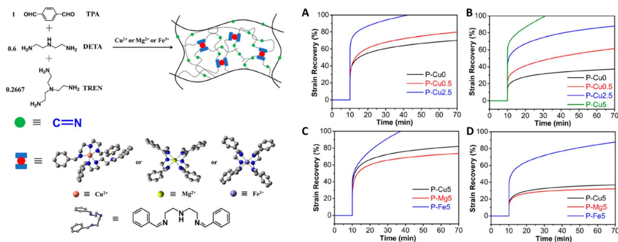
Fig. 6 (Left) Polyimine–metal complex vitrimers synthesized from terephthalaldehyde (TPA), diethylenetriamine (DETA), and tris(2-aminoethyl) amine (TREN). (Right) Strain recovery curves to show the creep response of the polyimine–metal complex vitrimers at (A) 60 \text{ }^\circ\text{C} , (B) 80 \text{ }^\circ\text{C} , (C) 100 \text{ }^\circ\text{C} , and (D) 120 \text{ }^\circ\text{C} . Adapted from ref. 127 with permission from the American Chemical Society, copyright 2020.
