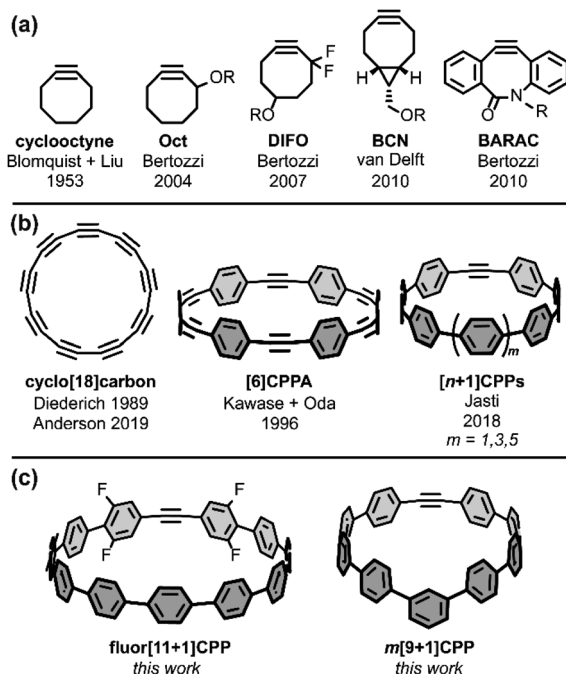
Fig. 1 (a) Examples of strained alkynes developed for copper-free click chemistry. (b) Strained alkynes in the field of carbon nanomaterials. (c) New strained alkyne-containing [ n +1]CPPs described in this work.
