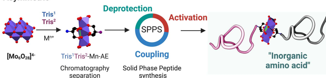
Fig. 8 Overview of the different synthetic routes currently available to produce covalent POM-peptide hybrids. (A) Structures of the POMs conjugated with peptides in the literature. (B) Tin-strategy has been described for lacunary Keggin and Wells-Dawson POMs. (C) TRIS-functionalization strategy. Above is described the symmetric derivatization of a Mn-AE POM via direct covalent conjugation or by the on-POM ring opening polymerization approach. Down is depicted how to prepare an asymmetric Mn-AE and its incorporation in a SPPS workflow as i-inorganic amino acid.
