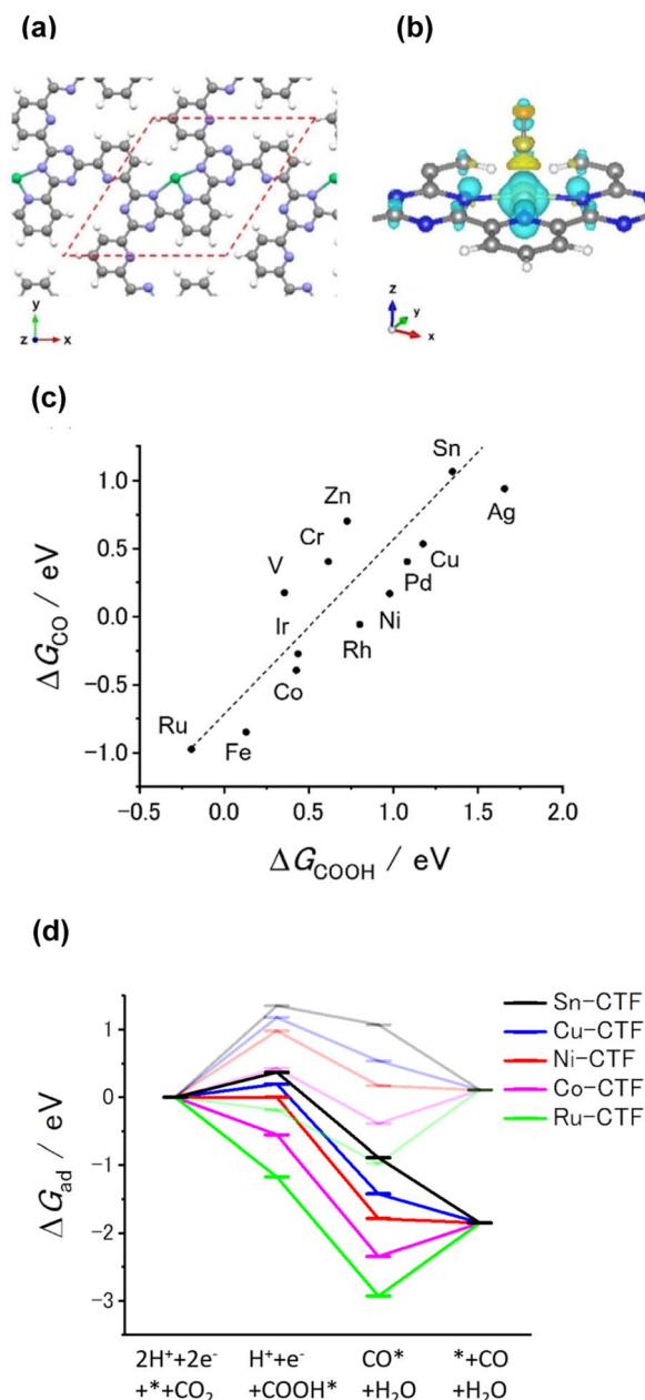
Fig. 1 (a) Optimized structure of Ni-CTF for DFT calculation (gray: C, white: H, blue: N, green: Ni). The red dashed line shows the unit cell. Approximately the same structure was obtained for all of the investigated M-CTFs. (b) Charge-density difference for Ni-CTF before and after COOH adsorption. The isosurface level is 0.003 e bohr −3 . The yellow and cyan areas represent regions of electron accumulation and depletion, respectively (gray: C, white: H, blue: N, green: Ni). (c) \Delta G_{CO} expressed in terms of \Delta G_{COOH} for each M-CTF. (d) Free energy diagrams for CO generation on Sn (black), Cu (blue), Ni (red), Co (purple), and Ru (green)-doped CTFs at 0 V (pale lines) and −0.98 V vs. CHE (dark lines).
