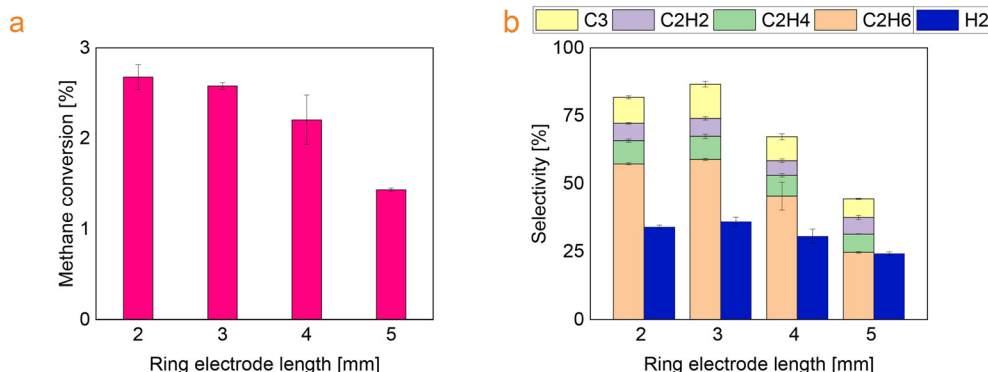
Fig. 8 (a) Methane conversion and (b) selectivity towards the main products as a function of ring electrode length.
