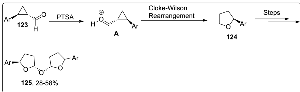
Scheme 38 Synthesis of oxybis(2-aryltetrahydrofuran) derivatives 125 via Cloke–Wilson rearrangement.
