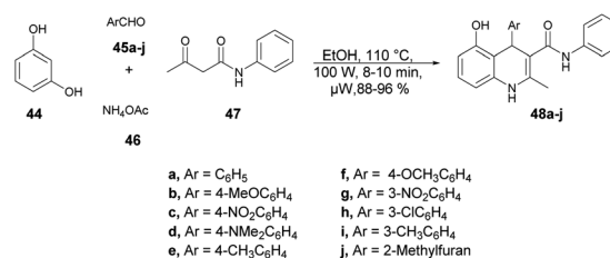
Scheme 16 Synthesis of 1,4-dihydroquinolines 48a–j .
