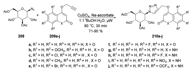
Scheme 73 Synthesis of triazole-linked N -glucopyranosides 210a-j .
