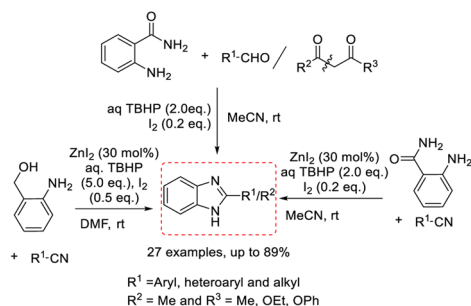
Scheme 144
