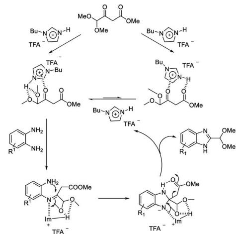
Scheme 90
