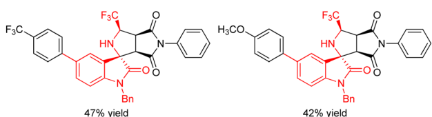
Scheme 6 Phase transfer-catalyzed stereoselective formation of spiro-fused [succinimide-pyrrolidine-oxindoles].
