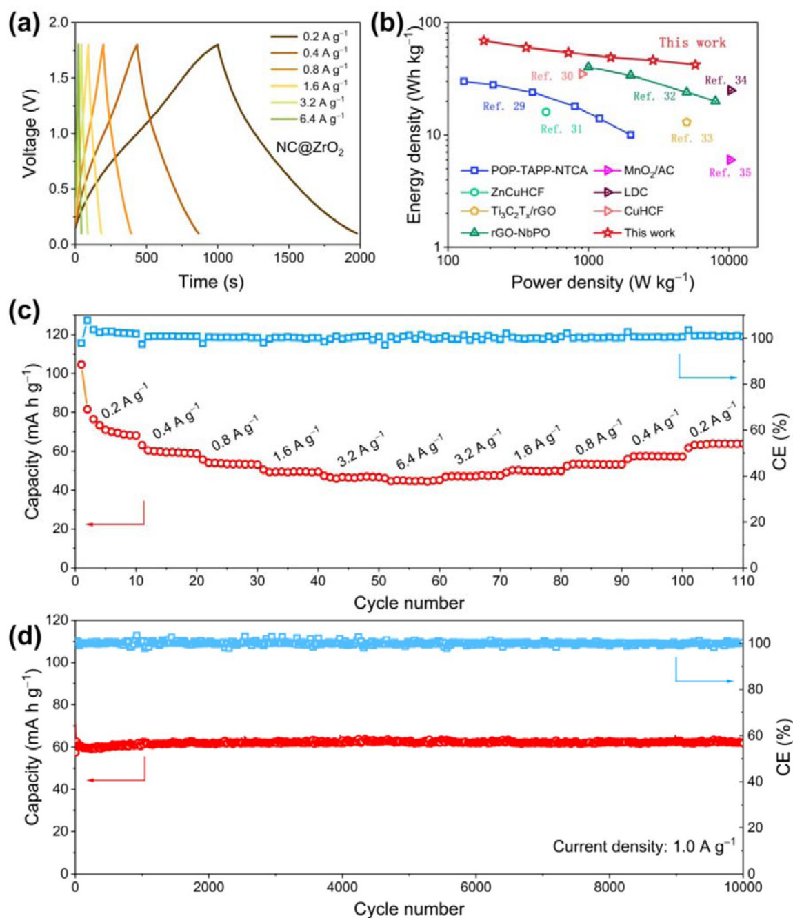
Fig. 5 Electrochemical performance of \text{NC@ZrO}_2 and \text{C@ZrO}_2 composite based ZHSs. (a) GCD curves of \text{NC@ZrO}_2 based ZHS at current ranging from 0.2 to 6.4 \text{A g}^{-1} . (b) The Ragone plot comparison between different supercapacitors and \text{NC@ZrO}_2 based ZHSs. (c) Rate properties of \text{NC@ZrO}_2 -based ZHS. (d) Cycling performance of \text{NC@ZrO}_2 -based ZHS.
