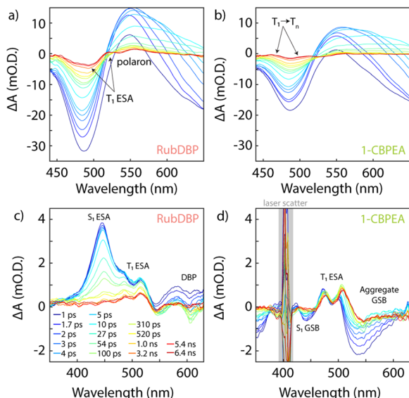
Fig. 4 Absorbance spectra from selected delay times for bilayer (a and b) under 700 nm pump and OSC only films (c and d) under 400 nm pump. (a) Transient absorbance spectra of FAMA/RubDBP bilayer film where the triplet ( T_1 ) excited state absorption (ESA) at 520 nm and polaron signal of rubrene at 550 nm are highlighted. (b) Absorbance spectra of a FAMA/1-CBPEA bilayer film with the T_1 \rightarrow T_n transitions at 460 nm and 510 nm of the 1-CBPEA annihilator shown. (c) RubDBP OSC only absorbance spectra where the singlet ( S_1 ) ESA at 445 nm and T_1 ESA spectral features at 485 nm and 515 nm corresponding to rubrene are observed as well as the DBP bleach at 600 nm. (d) 1-CBPEA OSC absorbance spectra where the S_1 ground state bleach (GSB) at 440 nm and T_1 ESA transitions at 470 nm and 510 nm are observed with an additional bleach feature at 530 nm. Grey box denotes pump laser scatter. Reproduced from ref. 60 with permission from the Royal Society of Chemistry, copyright 2022.
