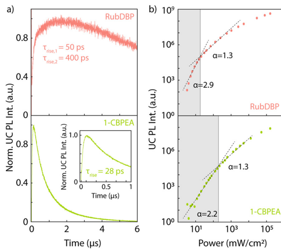
Fig. 5 (a) Normalized upconverted PL dynamics for FAMA/RubDBP (top) and FAMA/1-CBPEA (bottom) bilayer films under 780 nm pulsed excitation (50 kHz, 120 mW cm -2 ). Extracted triplet rise times are included for both, and smaller inset magnifies the quick rise of 1-CBPEA. (b) Power dependent upconverted emission for both FAMA/RubDBP (top) and FAMA/1-CBPEA (bottom) bilayer films with the corresponding extracted slopes (grey dashed lines) included. The calculated intensity threshold for each bilayer film were calculated from the intersection of the two fits (18.2 mW cm -2 for RubDBP and 192 mW cm -2 for 1-CBPEA). Reproduced from ref. 60 with permission from the Royal Society of Chemistry, copyright 2022.
