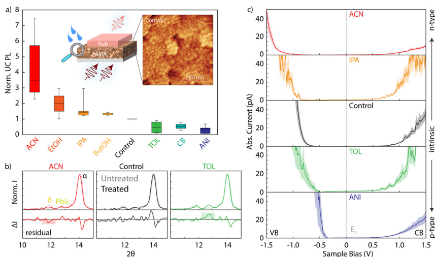
Fig. 9 (a) Box plots of upconverted PL intensities under 780 nm excitation. The spectra were integrated from 500 nm to 610 nm across numerous spots for the solvent treated FAMA/Rub bilayer films and normalized to the UC PL intensity of the untreated FAMA/Rub control for comparison. The inset shows the device structure and a scanning tunneling microscopy topography of the FAMA control film taken at -0.8 V and -100 pA. (b) Grazing incidence X-ray diffraction for the acetonitrile (ACN), control, and toluene (TOL) treated perovskite only films pre- (lighter shade) and post-solvent treatment (darker shade). Patterns were normalized to the perovskite (110) peak at 14^\circ to aid comparison. The residuals highlight the change after the solvent treatment. (c) Average scanning tunneling spectroscopy (STS) IV curves for the solvent treated perovskite only films. Shaded regions depict the 95% confidence interval for each sample set. All curves were measured from -2.0 to 2.0 V at a rate of 1.0 V s^{-1} . The tip was set to a bias of -1.5 V and setpoint current of -100 pA and stabilized between each IV spectra. Adapted with permission from ref. 144. Copyright 2022 John Wiley and Sons.
