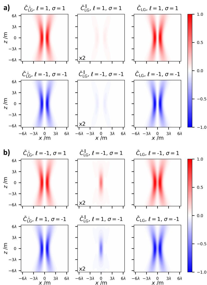
Fig. 6 Diffractive properties of the (left) transverse, \tilde{C}_{\text{LG}}^{\perp} , (centre) longitudinal, \tilde{C}_{\text{LG}}^{\parallel} , and (right) combined, \tilde{C}_{\text{LG}} , field contributions to the optical chirality densities of circularly polarised \sigma = \pm 1 LG ( \ell = \pm 1 , p = 0 ) beams, normalised to the total, \tilde{C}_{\text{LG}} . (a) Parallel SAM and OAM, \text{sgn } \ell = \text{sgn } \sigma . (b) Anti-parallel SAM and OAM \text{sgn } \ell \neq \text{sgn } \sigma . In all plots w_0 = \lambda .
