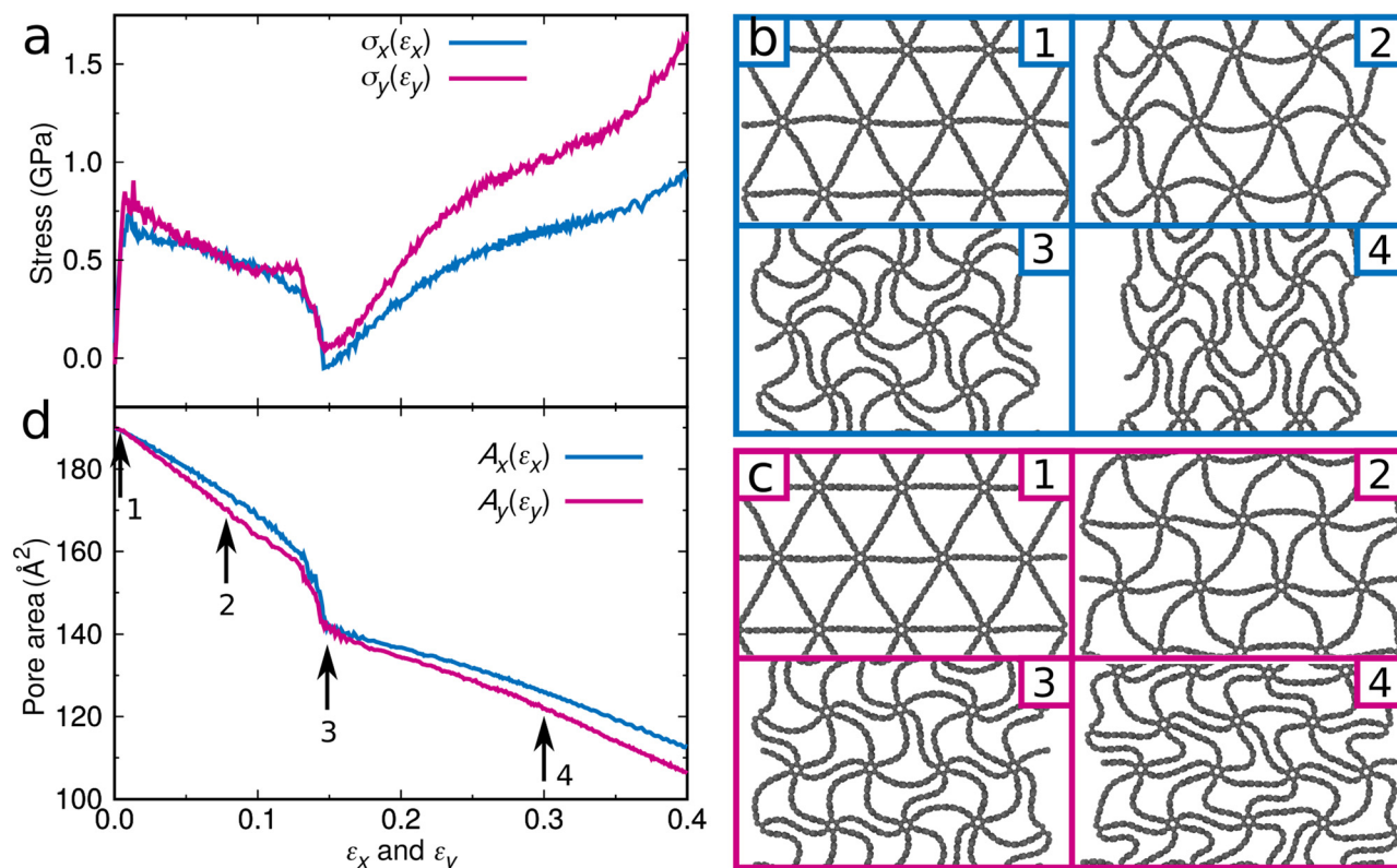
Fig. 2 Graphene foam membrane with an initial pore area of 187 Å 2 : (a) Stress-strain curves for loading in the x - and y -directions. Structure under increasing strain (0.005, 0.075, 0.150, and 0.300) applied in the (b) x - and (c) y -directions. (d) Pore area as a function of the strain applied in the x - and y -directions.
