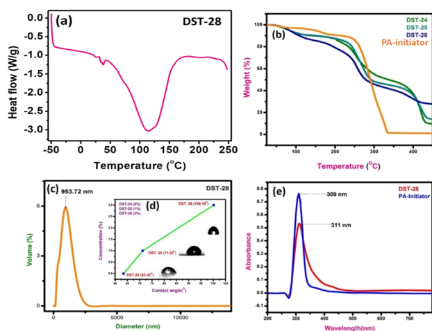
Fig. 3 (a) Differential scanning calorimetry (DSC) thermogram of DST-28 (enthalpy: 599.51 J \text{g}^{-1} , 10 °C \text{min}^{-1} ), (b) thermogravimetric analysis (TGA) of various percentages of polymer composites: DST-24 (phenoxyaniline- b -PMMA, without clay), DST-25 (1% clay containing phenoxyaniline- b -PMMA) and phenoxyaniline initiator, (c) particle size analysis of DST-28 (3% clay containing phenoxyaniline- b -PMMA), (d) contact angle measurements of different percentages of composites: DST-24 (phenoxyaniline- b -PMMA, without clay), DST-25 (1% clay containing phenoxyaniline- b -PMMA), DST-28 (3% clay containing phenoxyaniline- b -PMMA) and (e) UV-vis spectra of the macroinitiator with the highest percentage of the composite (DST-28 with 3% clay).
