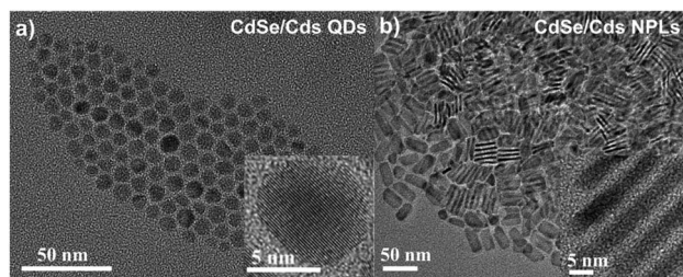
Fig. 1 (a) TEM image (50 nm) of CdSe/CdS QDs with a 5 ML shell, where the HRTEM image (5 nm) of a CdSe/CdS QDs and the corresponding fast Fourier transform pattern is shown in the inset on the right-bottom corner. (b) TEM image (50 nm) of CdSe/CdS NPLs with a 4 ML shell.
